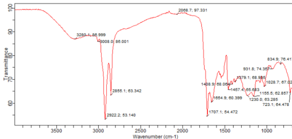
Figure 2b: FT-IR spectrum for silica (GN)
