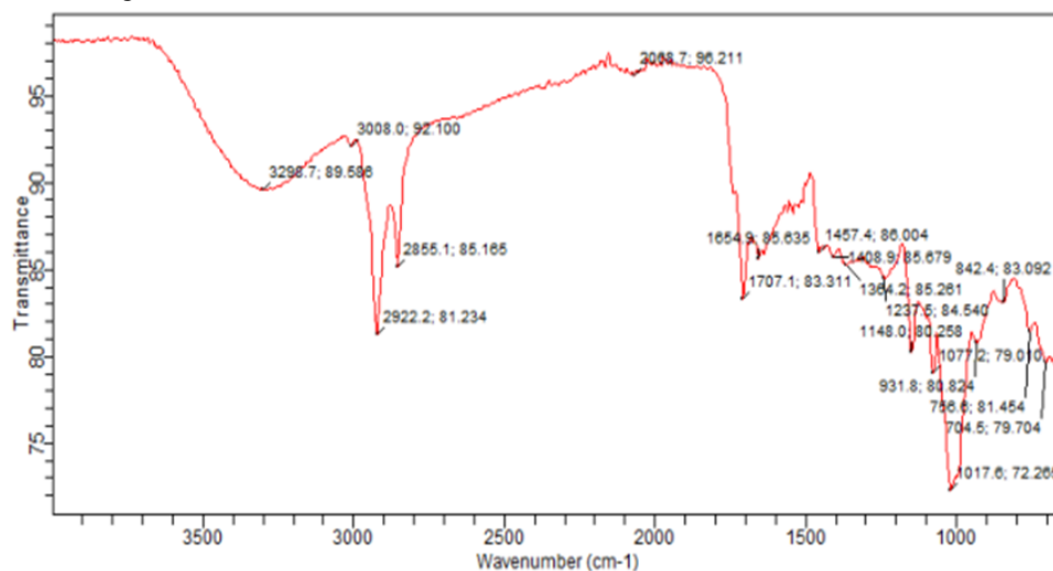
Figure 2a: FT-IR spectrum for silica (BN)
