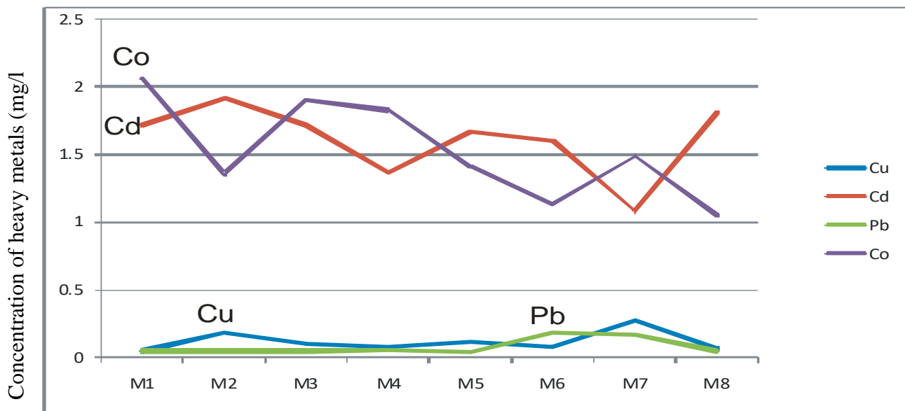
Figure 6: Trend of accumulation of heavy metals at sampling point 4 in Wulmi River
