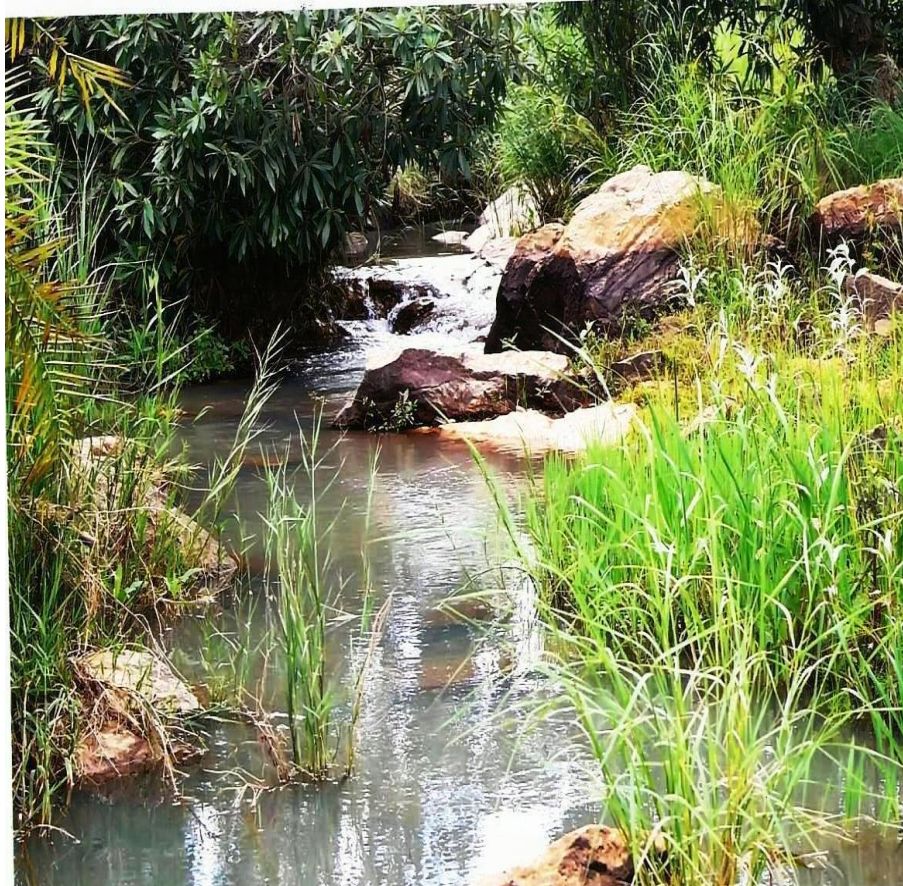
Figure 1: Plate I: Wulmi River in Pankshin Local Government of Plateau State
