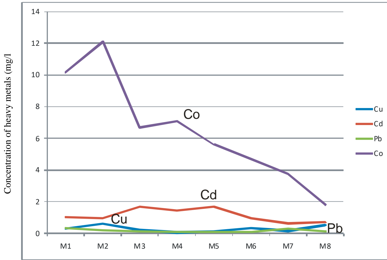
Figure 3: Trend of accumulation of heavy metals at sampling point 1 in Wulmi River
