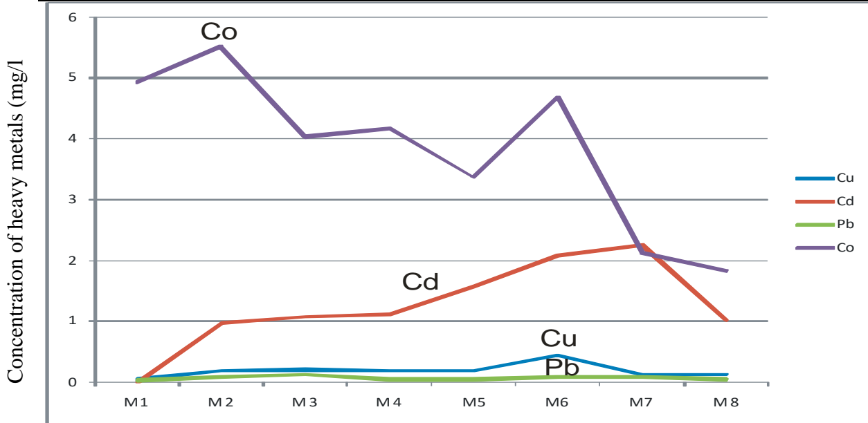
Figure 4: Trend of accumulation of heavy metals at sampling point 2 in Wulmi River
